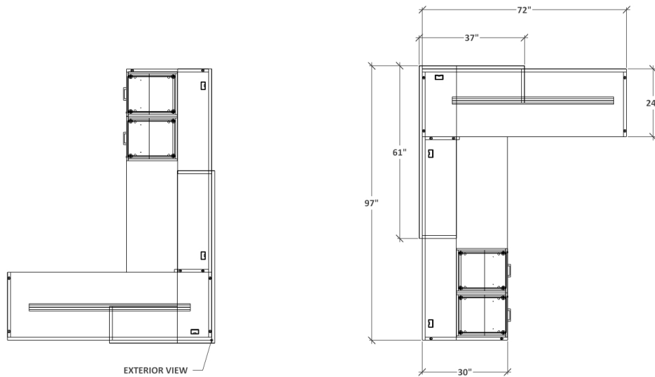
EXTERIOR VIEW
